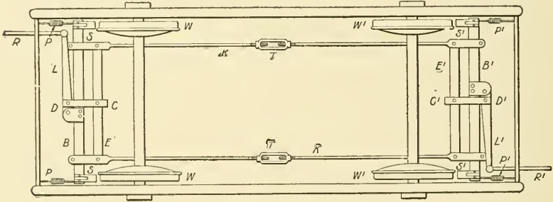
Fig. 81. Brake Rigging for Single-Truck Car
